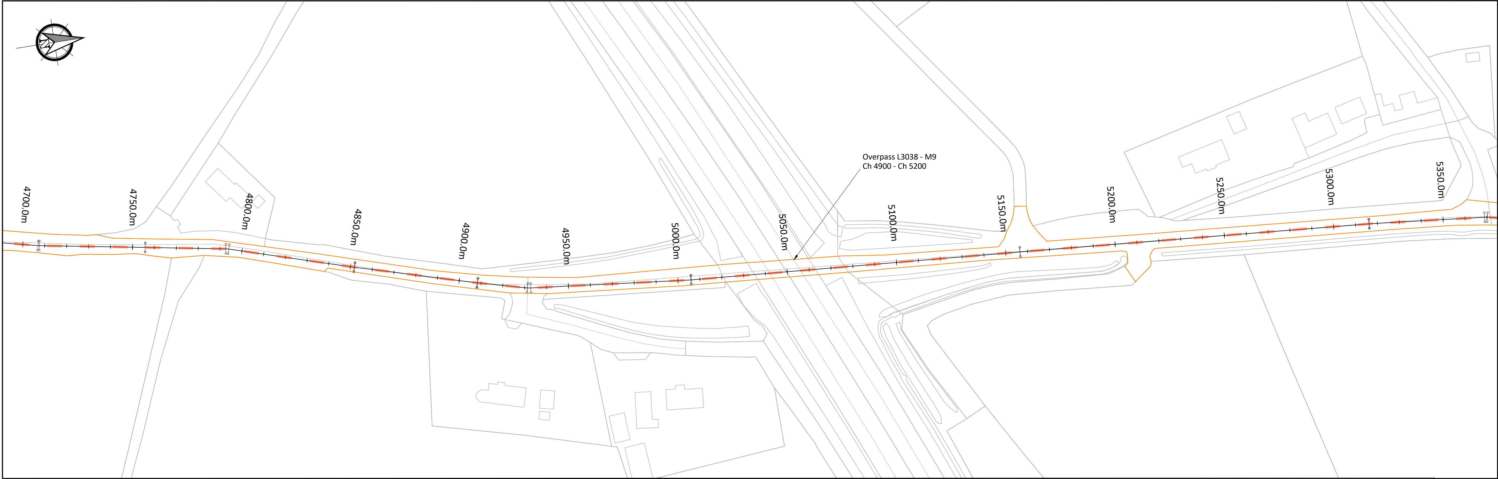
GRID CONNECTION ROUTE 4700.0M - 5350.0M Scale 1:1000
